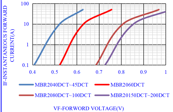
Fig.2- TYPICAL INSTANTANEOUS FORWARD
