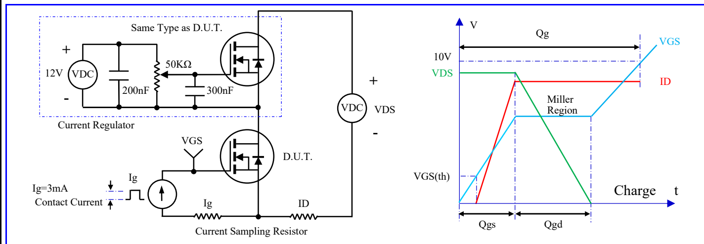
Fig.15-Gate Charge Test Circuit & Waveform
