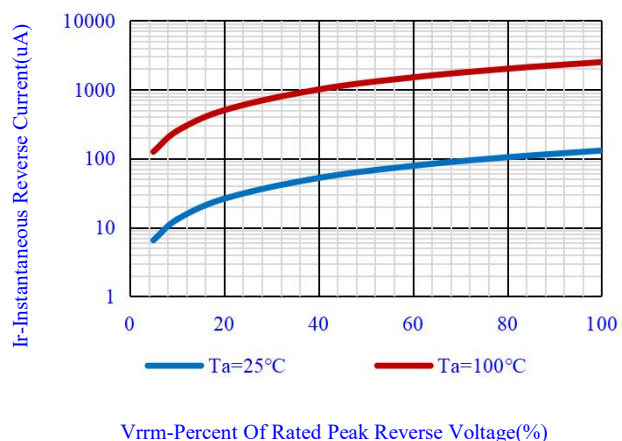
Fig.3-Typical Reverse Characteristics
