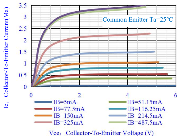
Fig.1-Static Characteristics
