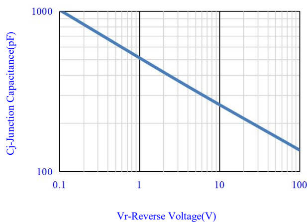
Fig.4-Typical Junction Capacitance
