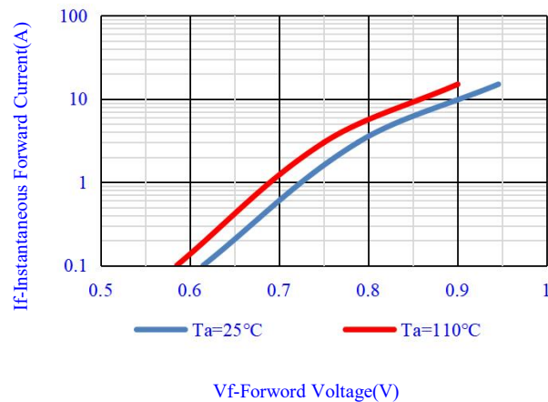
Fig.2-Typical Instantaneous Forward
