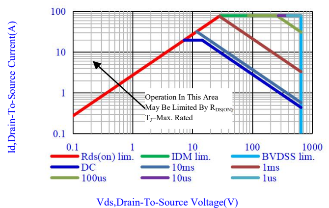
Fig.12-Maximum Safe Operating Area(SOA)
