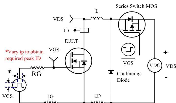
Fig.16- Unclamped Inductive Switching (UIS) Test Circuit & Waveform
