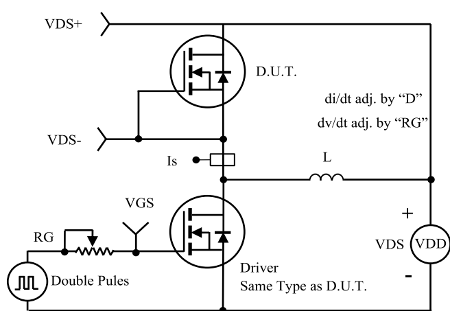
Fig.17- Diode Recovery Test Circuit & Waveform
