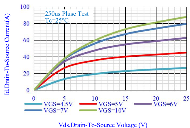
Fig.1-Output Characteristics
