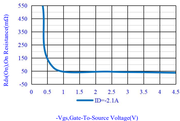
Fig.4-On Resistance Vs. Gate Source Voltage
