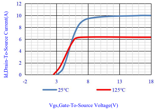
Fig.8-Transfer Characteristics
