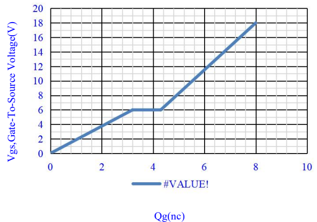
Fig.16-Gate Charge Waveform
