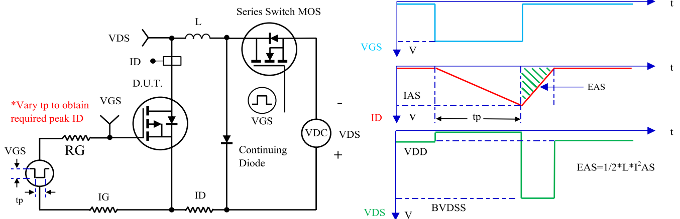
Fig.16- Unclamped Inductive Switching (UIS) Test Circuit & Waveform
