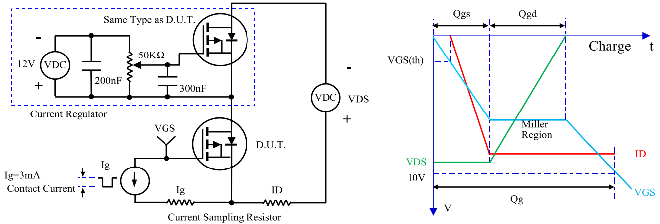
Fig.15- Gate Charge Test Circuit & Waveform
