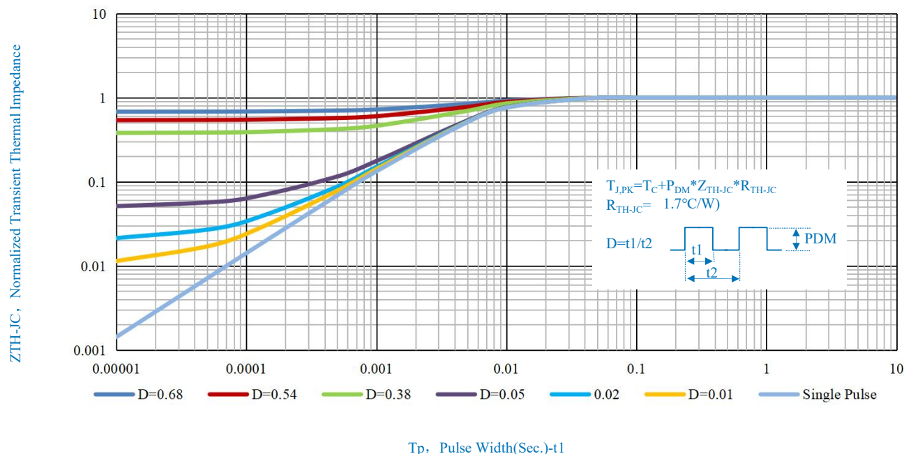
Fig.13- Normalized Maximum Transient Thermal Impedance Vs.Pulse Width
