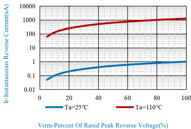
Fig.3-Typical Reverse Characteristics
