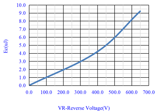
Fig.8-Capacitance Stored Energy
