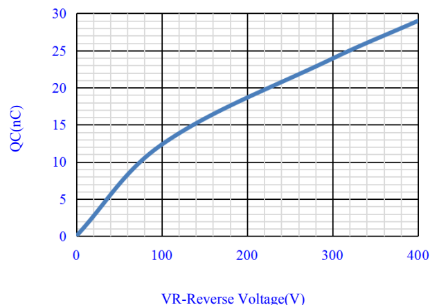
Fig.6-Total Capacitance Charge Characteristics vs. Reverse Voltage
