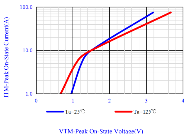
Fig.3-On-State Characteristics
