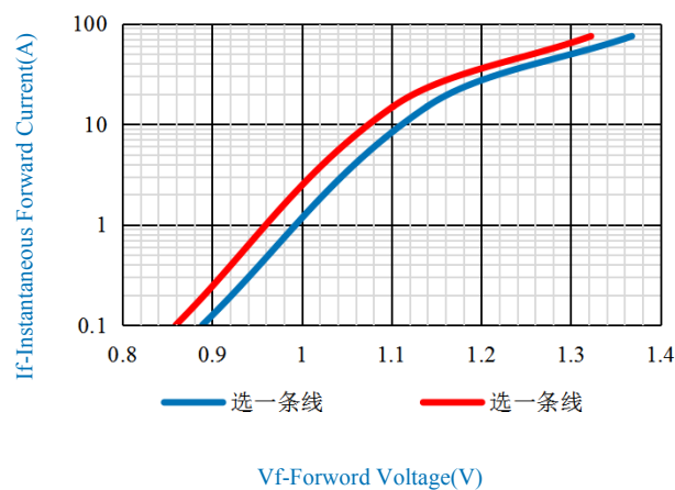
Fig.2-Typical Instantaneous Forward
