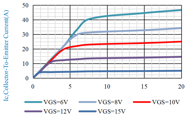
Fig.2-Output Characteristics@Tj=175°C
