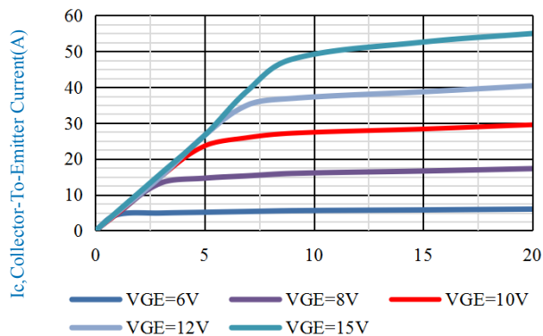
Fig.1-Output Characteristics@Tj=25°C
