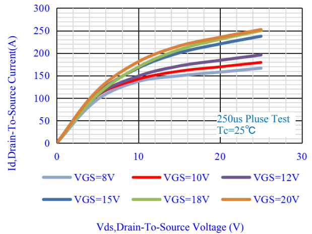
Fig.2-Output Characteristics@Tj=175°C
